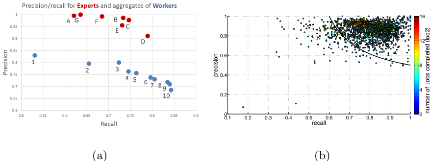
Fig. 4: (a) Precision and recall of experts (red) and the majority vote of AMT workers (blue). Note that the aggregate of 3 workers has better or similar recall to most experts. (b) illustrates the precision and recall of workers, with color indicating how many jobs they completed. For details and definition of ground truth for each plot see text.
